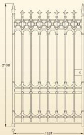
GA114 Stirling pedestrian gate (4ft single gate, 178kg)
