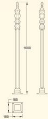
GA122 Stirling half height railing post (40kg)
