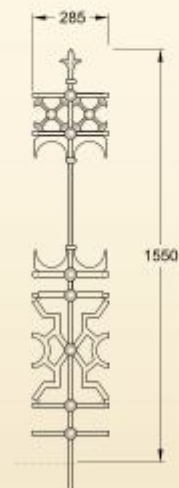
GA018 Stewart full height railing joiner panel with root fixing (18kg)
